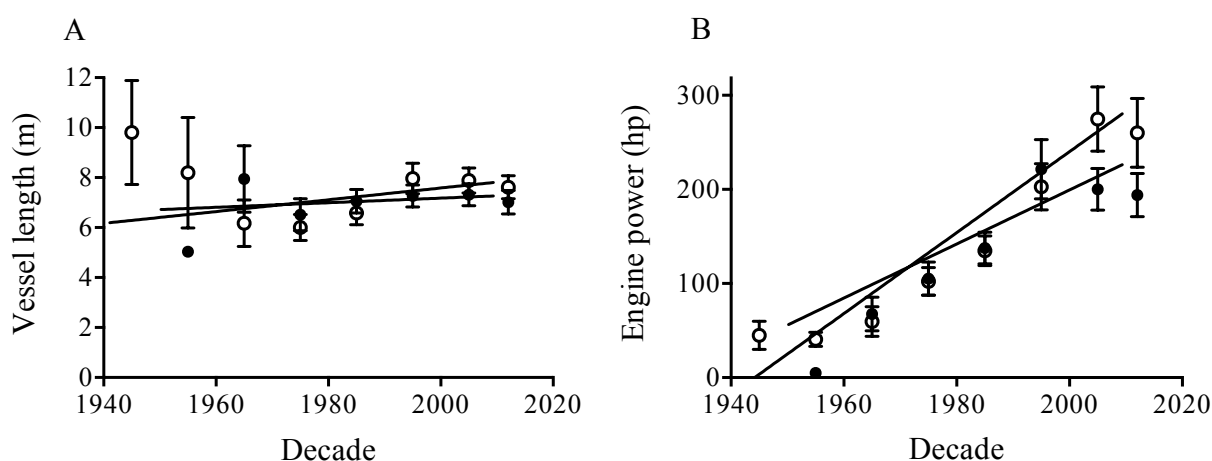
Figure 6. Changes in vessel length and engine power over time, by sector. A) Average vessel length and B) engine power by decade. Open circles show recreational (including charter) fishers, closed circles show commercial fishers recall. Vertical lines show the standard error, horizontal lines show the linear regression.
