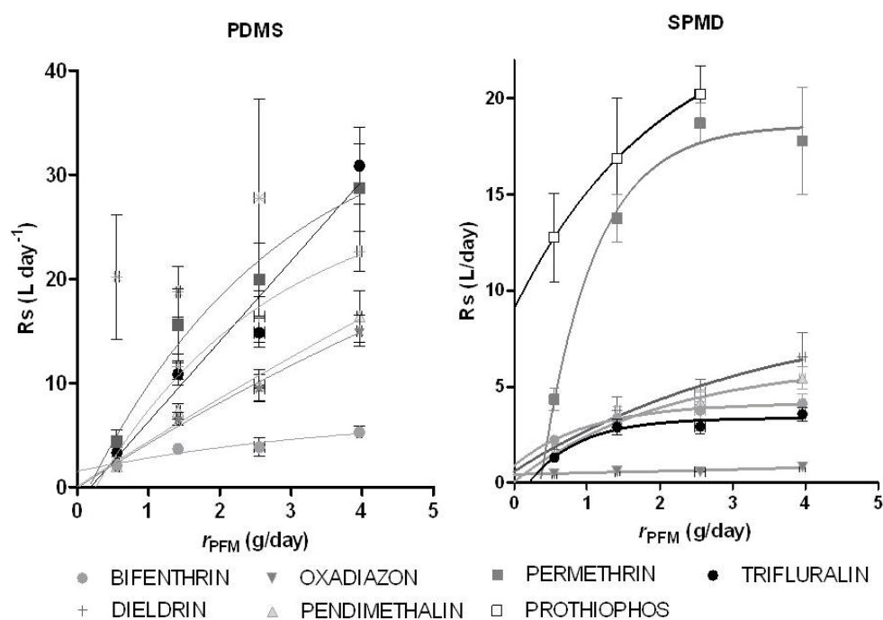
Figure 3.7. PDMS and SPMD sampling rates ( R_s ) as a function of water velocity r_{PFM}
